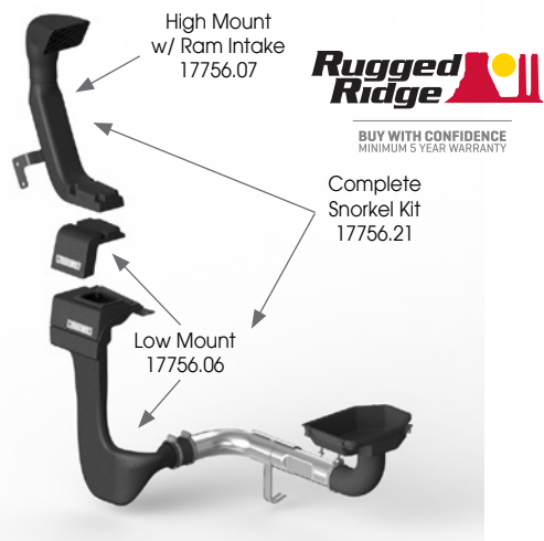
HIGH MOUNT W/ RAM INTAKE
